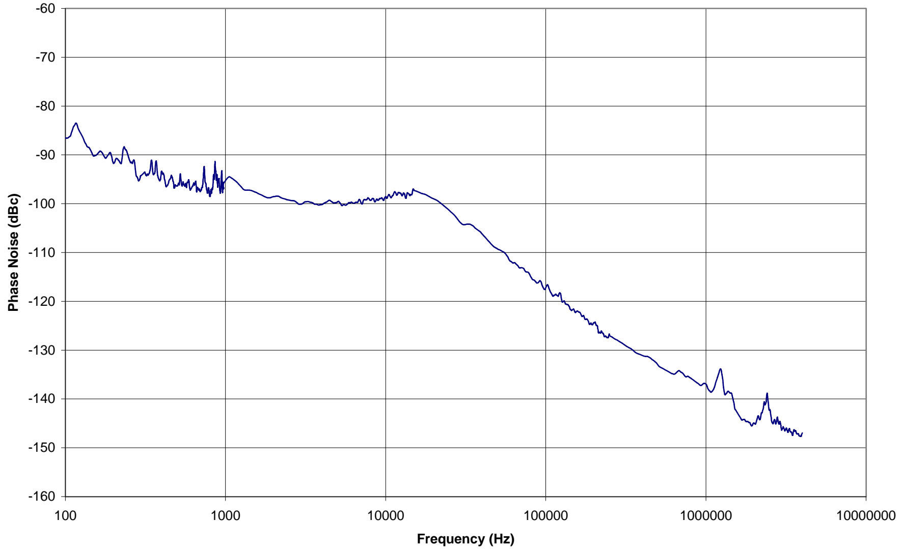
12.8GHz Single Loop PLDRO w External 10MHz reference
